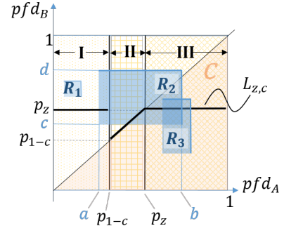
Figure G.23: Half-open rectangles and the three regions defined by L_{z,c} . The probability that F^* – a pre-(probability)measure – assigns to a half-open rectangle, is computed by summing the probability contributions from the rectangle's intersection with each of regions I , II , III and L_{z,c} . On each rectangle, the difference between F_k^* and F^* can be made vanishingly small as k \rightarrow \infty . We show that this convergence is uniform on the set \mathcal{R} of half-open rectangles.
