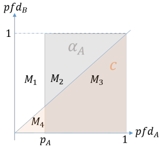
Figure 3: Any joint prior distribution F must satisfy M_2 + M_3 = \alpha_A and M_4 + M_3 = c , where F assigns probability M_i to region i .
