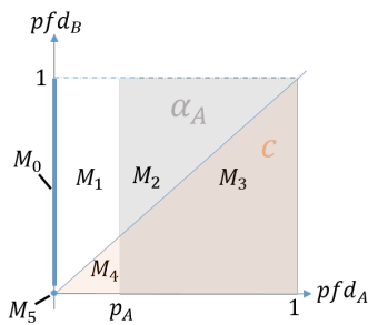
Figure 7: An allocation of probabilities for any prior distribution that satisfies (4), (6) and (13). That is, M_5 + M_4 + M_3 = c , M_3 + M_2 = \alpha_A , and M_5 + M_0 = \theta_A , where M_i is the probability associated with the depicted i -th subset of the unit square. Note, the mass M_5 is assigned to (0,0) , while M_0 is assigned to the segment \{(0,y) | 0 < y \leq 1\} .
